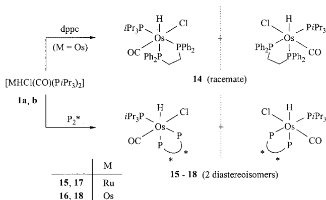
Scheme 4. [ 15, 16 : P_2^* = (S,S) -Chiraphos; 17, 18 : P_2^* = (S,S) -Diop]
