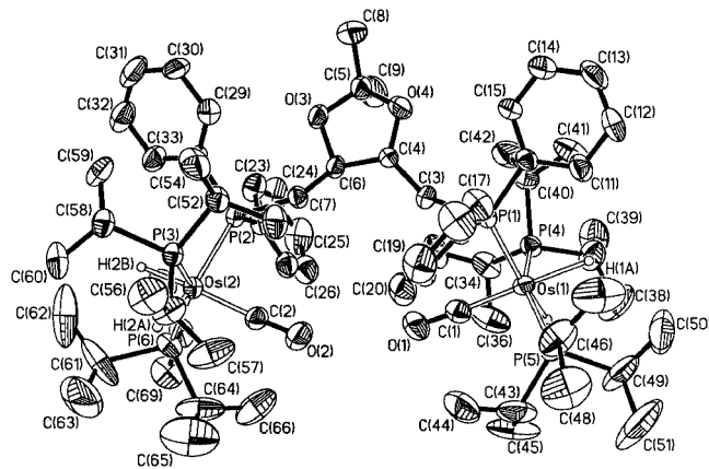
Figure 1. Molecular structure of compound 22 ; selected bond lengths (Å) and angles ( ^\circ ): Os(1)–P(1) 2.3725(13), Os(2)–P(2) 2.3711(4), Os(2)–P(3) 2.3431(16), Os(1)–P(4) 2.3412(15), Os(1)–P(5) 2.3457(15), Os(2)–P(6) 2.3640(15), Os(1)–C(1) 1.873(7), Os(2)–C(2) 1.852(6), C(1)–O(1) 1.197(7), C(2)–O(2) 1.191(7); P(1)–Os(1)–P(4) 101.27(5), P(1)–Os(1)–P(5) 106.24(6), P(1)–Os(1)–C(1) 88.51(19), P(4)–Os(1)–P(5) 148.90(6), P(4)–Os(1)–C(1) 97.9(2), P(5)–Os(1)–C(1) 97.0(2), P(2)–Os(2)–P(3) 101.59(5), P(2)–Os(2)–P(6) 109.33(5), P(2)–Os(2)–C(2) 91.31(18), P(3)–Os(2)–P(6) 145.65(5), P(3)–Os(2)–C(2) 96.42(18), P(6)–Os(2)–C(2) 97.44(18), P(1)–C(3)–C(4) 126.2(4), P(2)–C(7)–C(6) 120.2(4), C(3)–C(4)–C(6) 110.7(4), C(7)–C(6)–C(4) 114.4(4), C(3)–C(4)–O(4) 113.1(5), C(7)–C(6)–O(3) 111.6(4), C(4)–O(4)–C(5) 111.4(4), C(6)–O(3)–C(5) 106.4(4).
