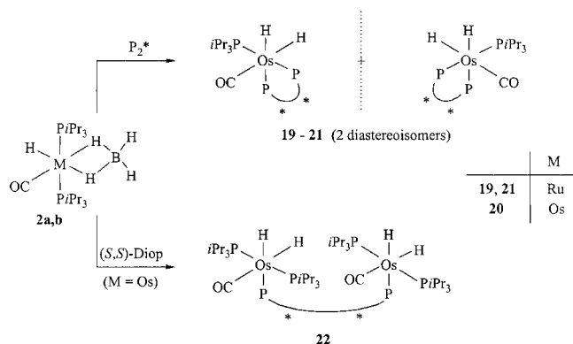
Scheme 5. [ 19 , 20 : P_2^* = (S,S) -Chiraphos; 21 , 22 : P_2^* = (S,S) -Diop]
